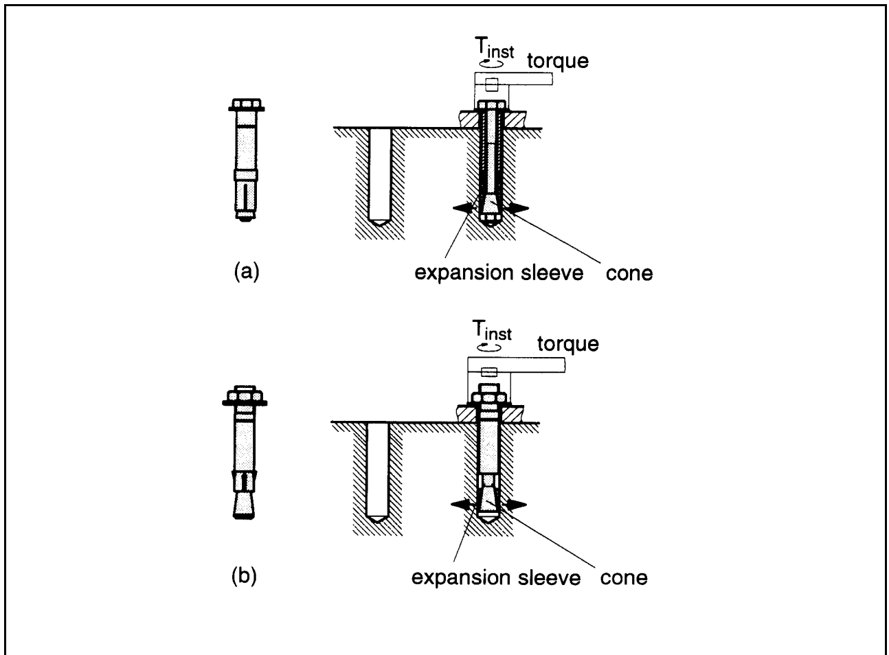
Figure 2.2 Examples of torque-controlled expansion anchors
